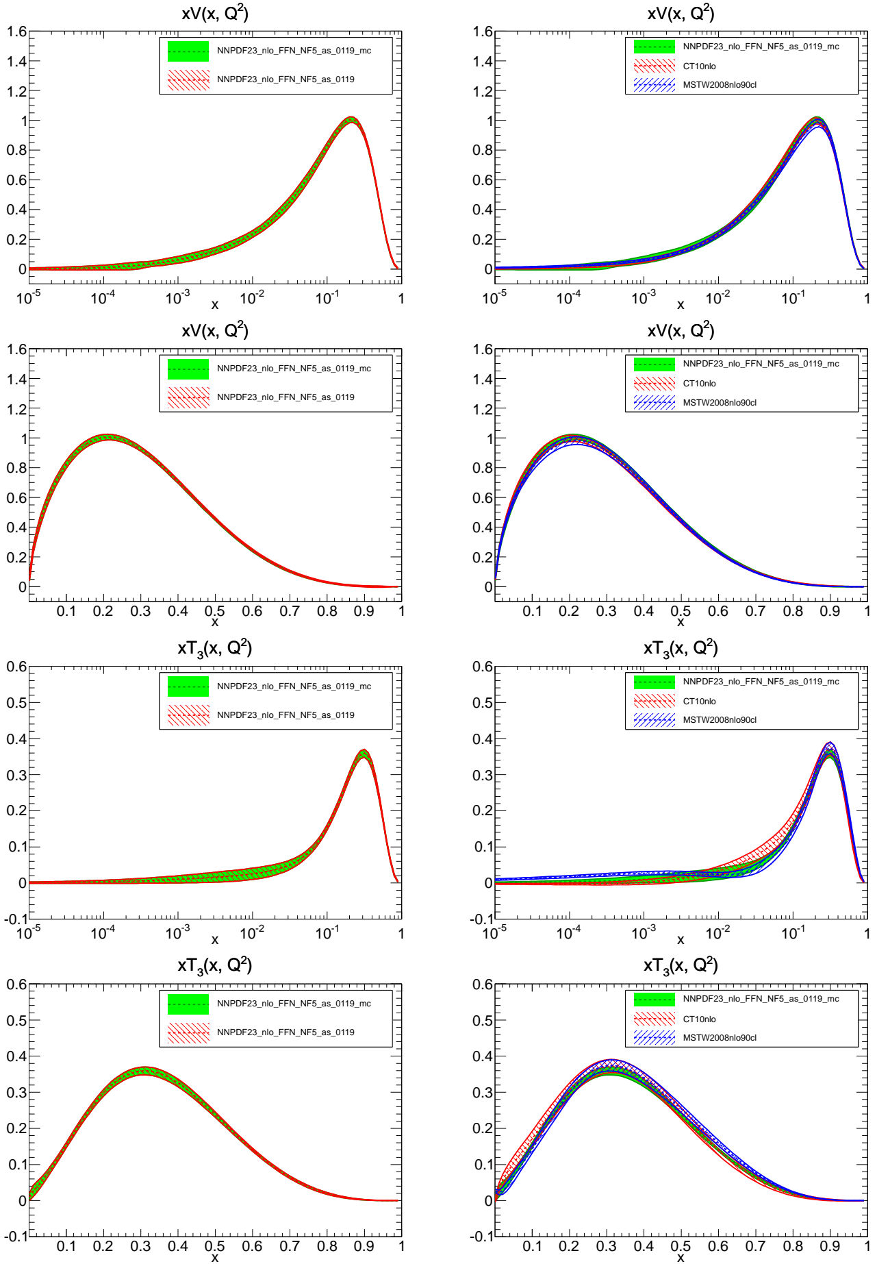
Figure 4: Comparison between PDFs at Q^2 = 2.0 \text{e} + 00 \text{ GeV}^2 .
