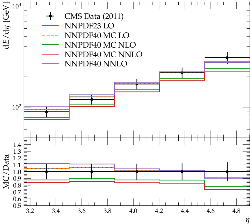
Energy flow in MB events at \sqrt{s} = 7 TeV
