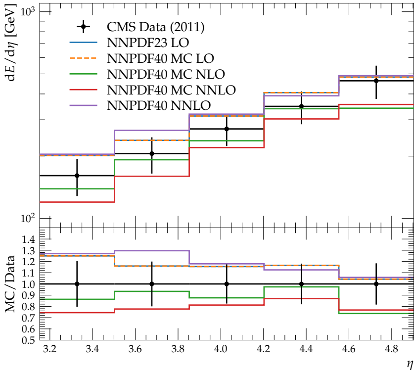
Energy flow in dijet events at \sqrt{s} = 7 TeV and p_{\perp}^{\text{jets}} > 20 GeV
