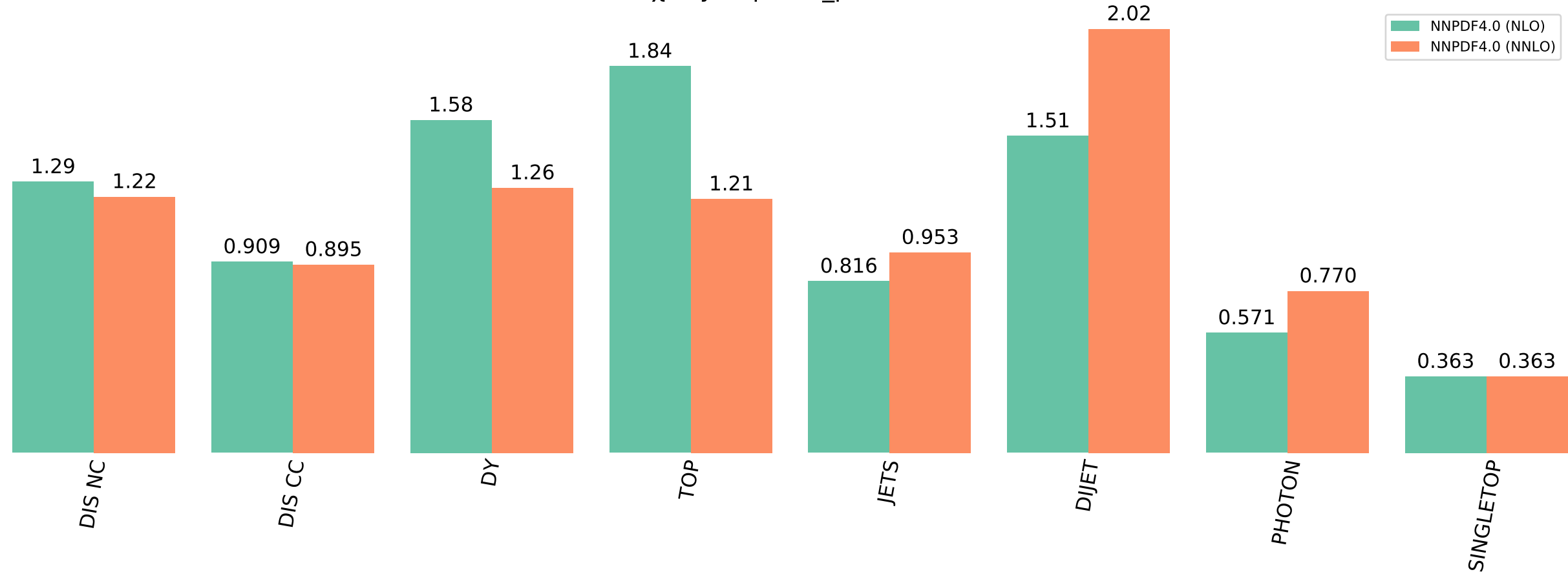
\chi^2 by nnpdf31_process
