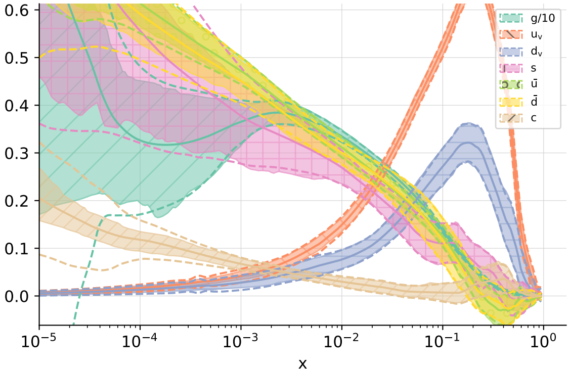
Collider only Q= 2.0 GeV
