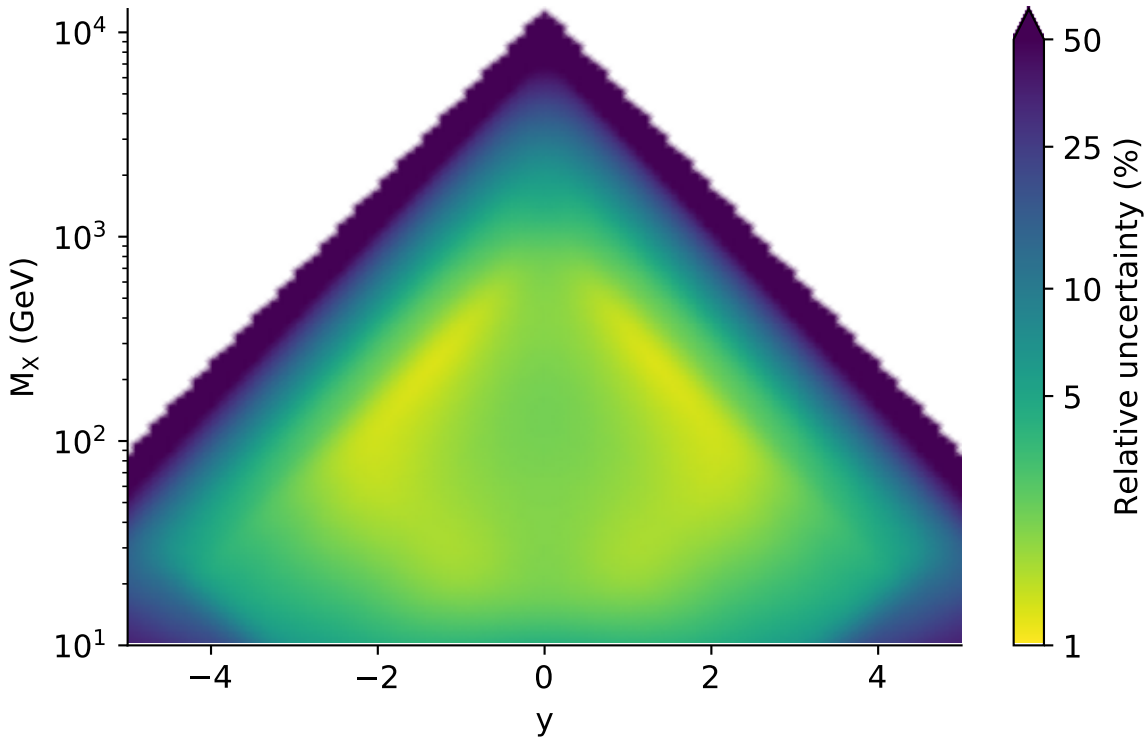
Relative uncertainty for gg-luminosity 3.0 dataset - \sqrt{s} = 13000.0 GeV
