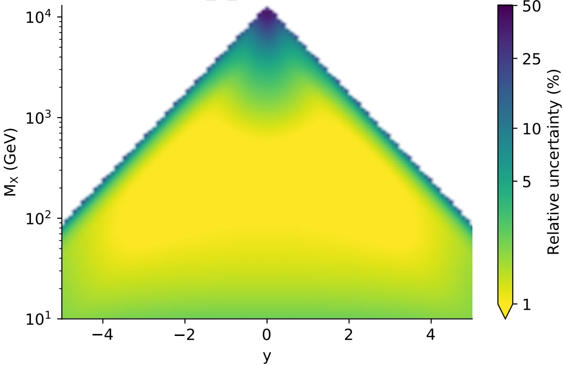
Relative uncertainty for q\bar{q} -luminosity ABMP16als118_5_nnlo - \sqrt{s} = 13000.0 GeV
