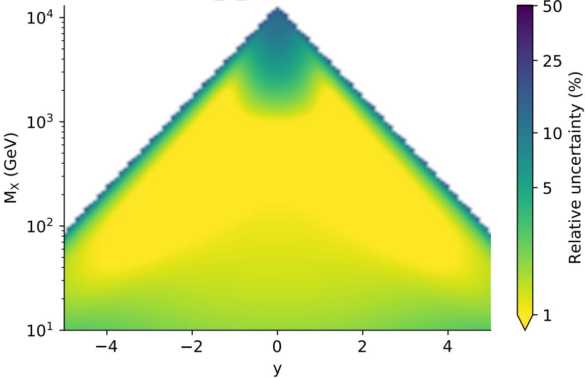
Relative uncertainty for qq-luminosity ABMP16als118_5_nnlo - \sqrt{s} = 13000.0 GeV
