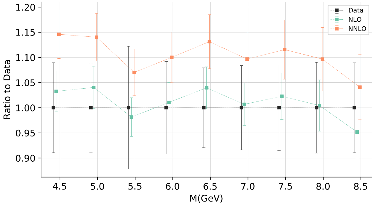
DY E886 \sigma_{DY}^p qplot = 7
