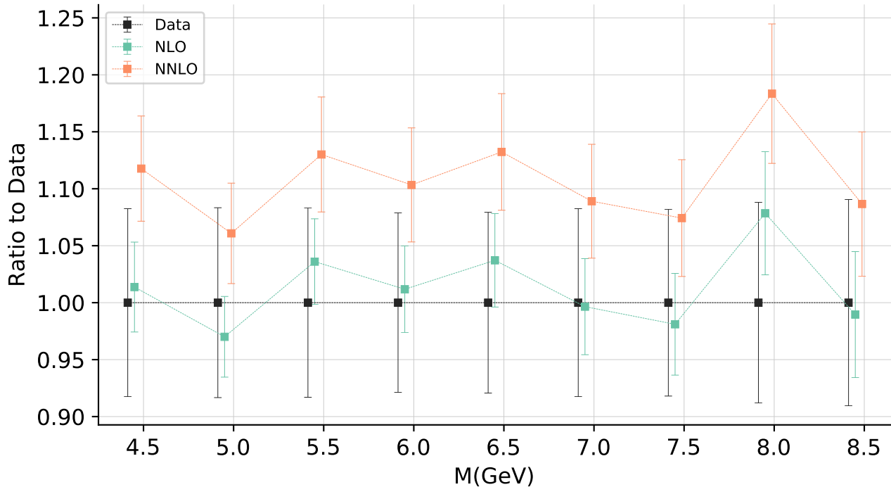
DY E886 \sigma_{DY}^p qplot = 6
