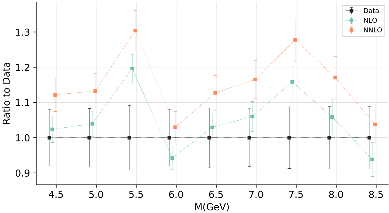
DY E886 \sigma_{DY}^p qplot = 5
