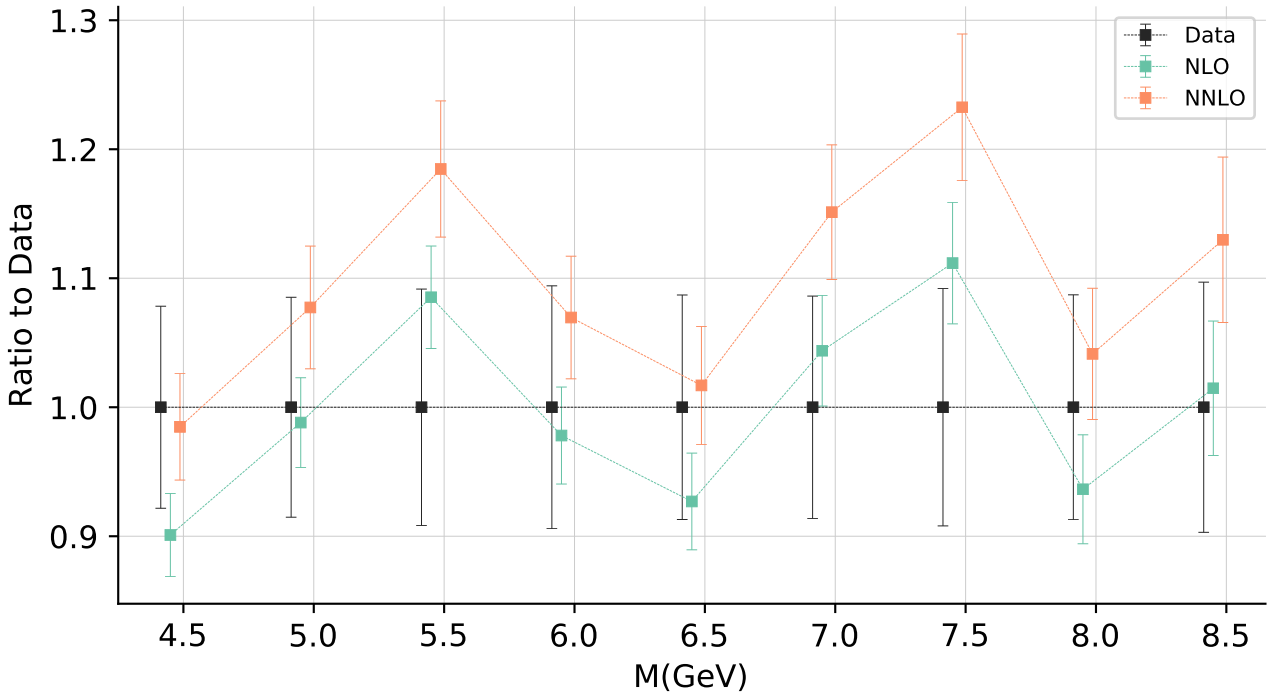
DY E886 \sigma_{DY}^p qplot = 4
