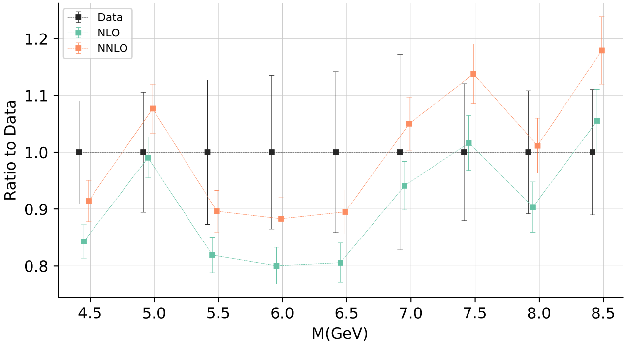
DY E886 \sigma_{DY}^p qplot = 2
