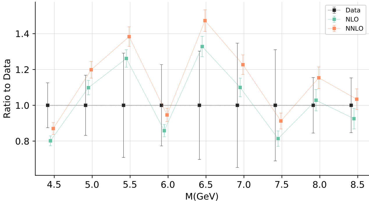
DY E886 \sigma_{DY}^p qplot = 1
