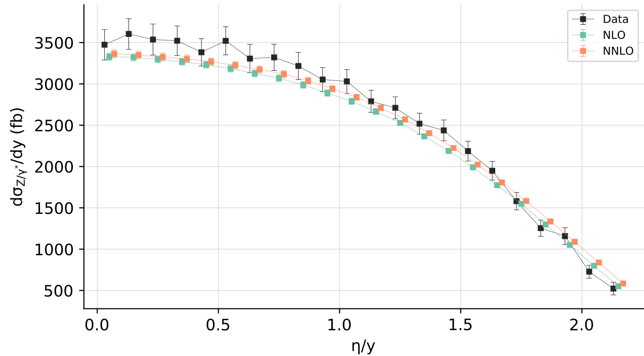
CMS Drell-Yan 2D 7 TeV 2011 M(GeV) = 160.0
