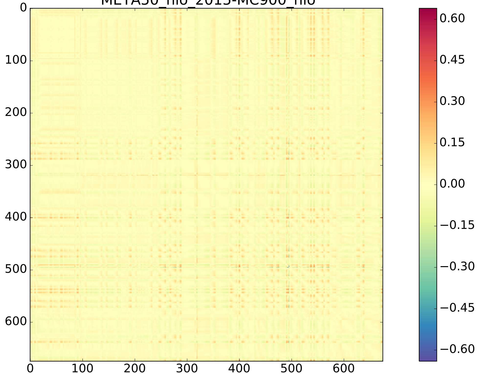
Observables correlation META50_nlo 2015-MC900_nlo
