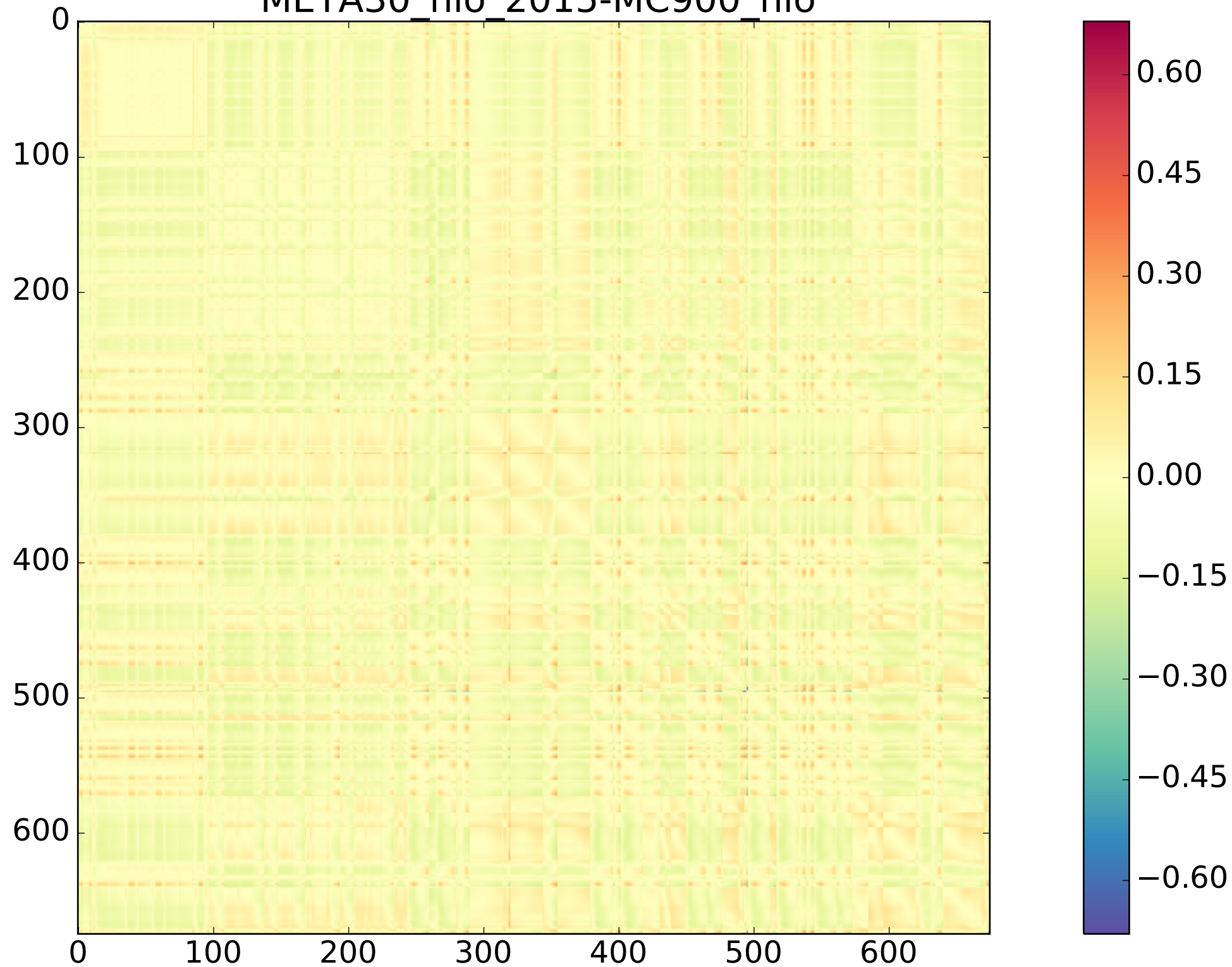
Observables correlation META30_nlo 2015-MC900_nlo
