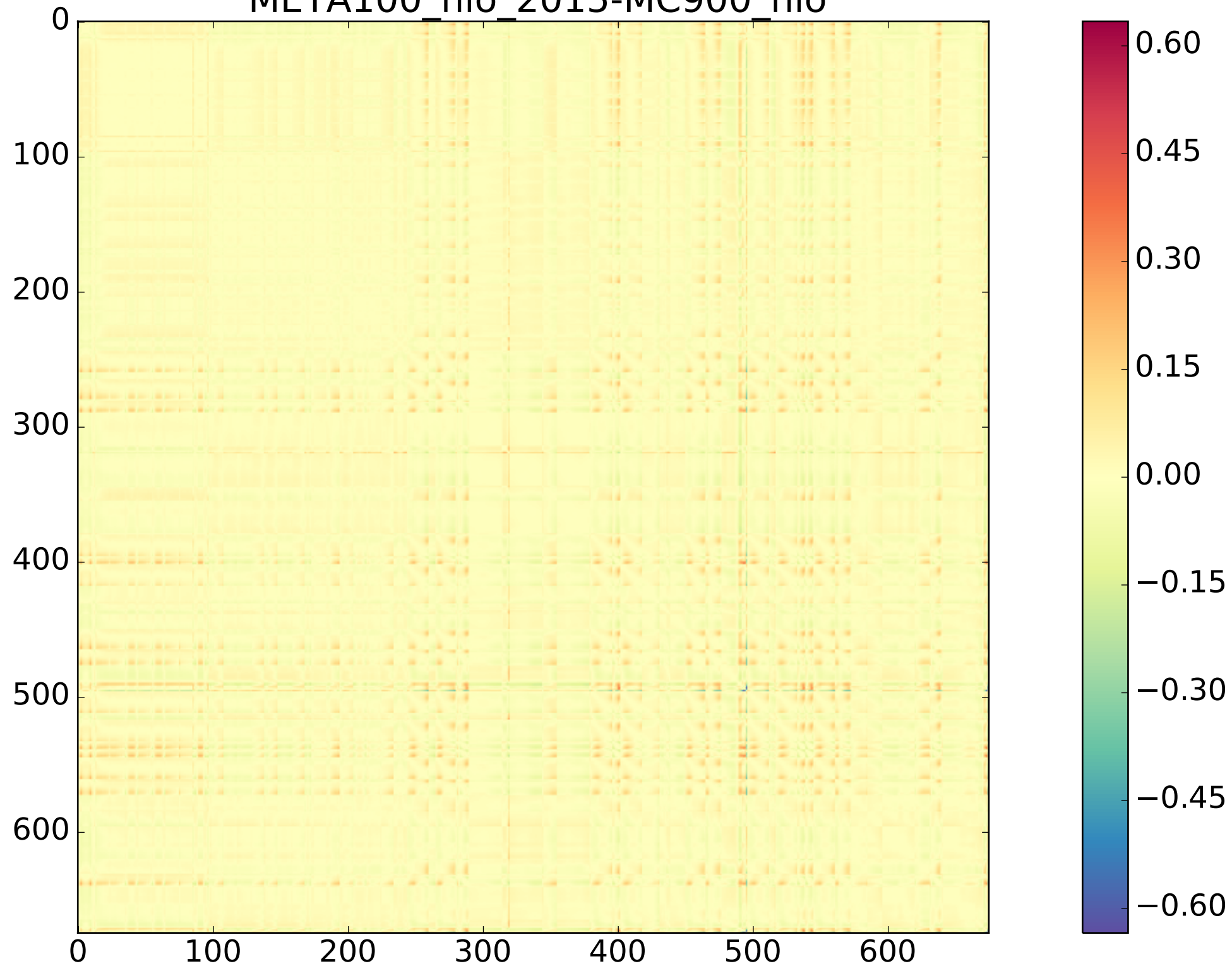
Observables correlation META100 nlo 2015-MC900 nlo
