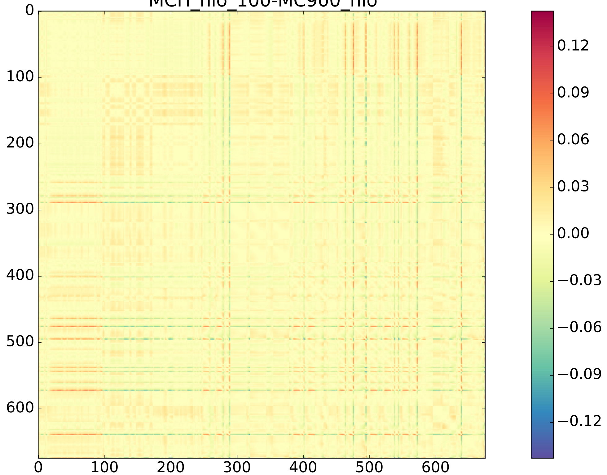
Observables correlation MCH_nlo_100-MC900_nlo
