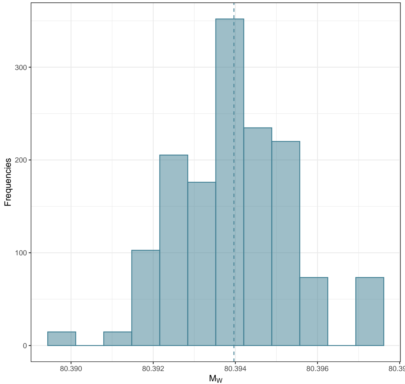
Mw Distr. 80.394 NNPDF31_nnlo_as_0118
