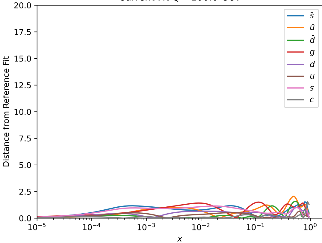
Current Fit Q= 100.0 GeV
