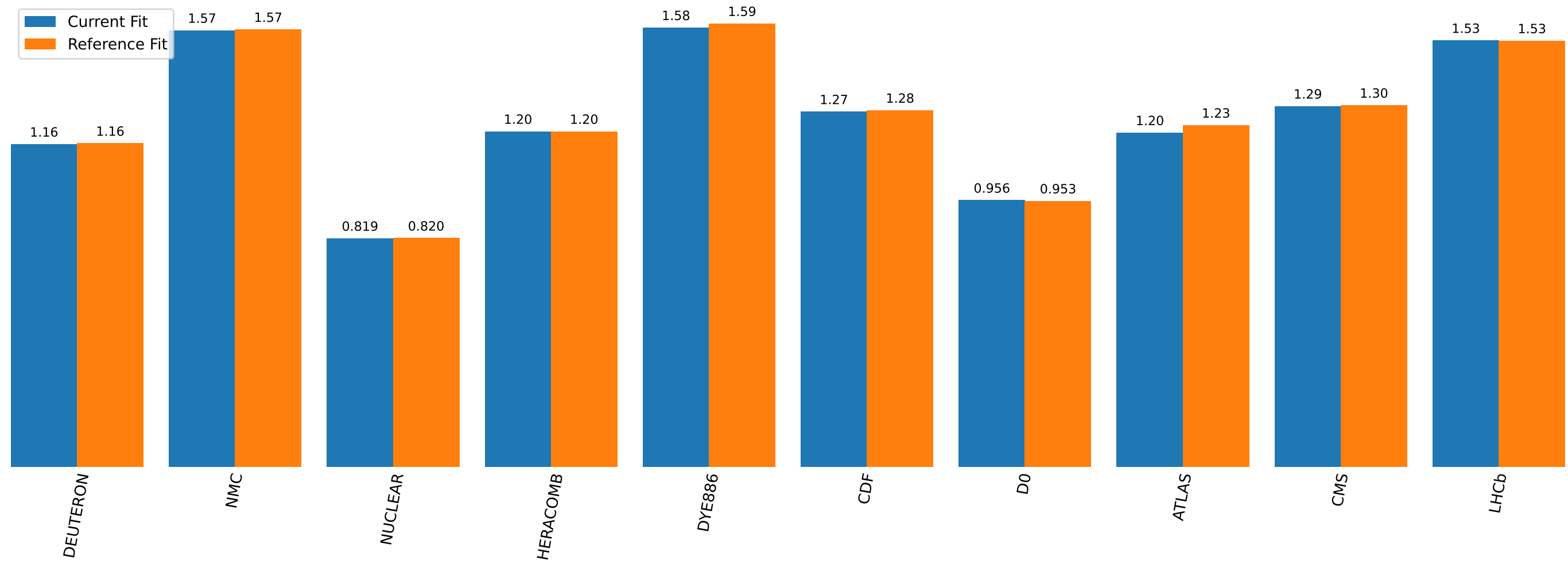
\chi^2 by experiment
