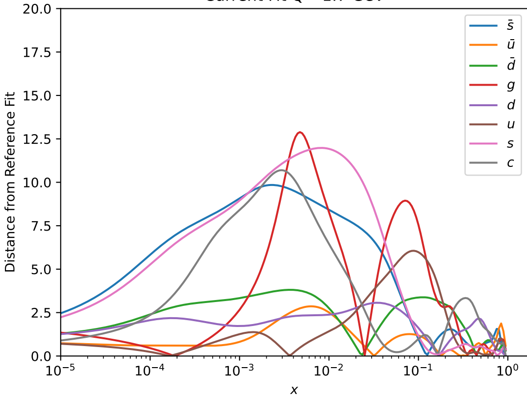
Current Fit Q= 1.7 GeV
