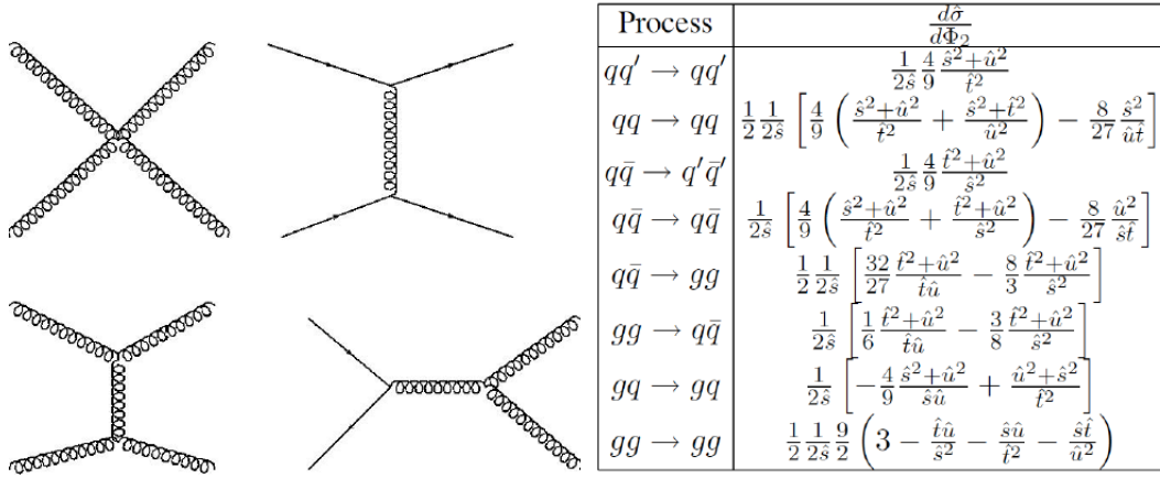
Figure 22: Left plot: a representative subset of the Feynman diagrams that contribute to the hadroproduction jet cross-section at the Born level. Right plot: the result for the partonic cross-sections for different scattering channels.
