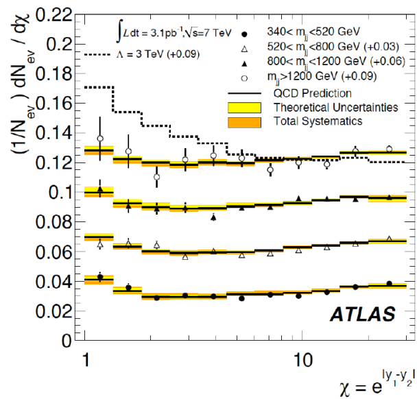
Figure 24: Measurement of the jet cross-section as a function of \chi , where the QCD predictions are compared to a model with quark substructure, characterized by a scale \Lambda = 3 \text{ TeV} .
