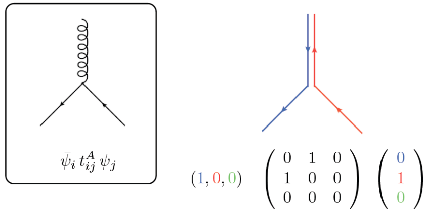
Figure 5: The emission of a gluon from a quark interpreted in terms of color flow.
