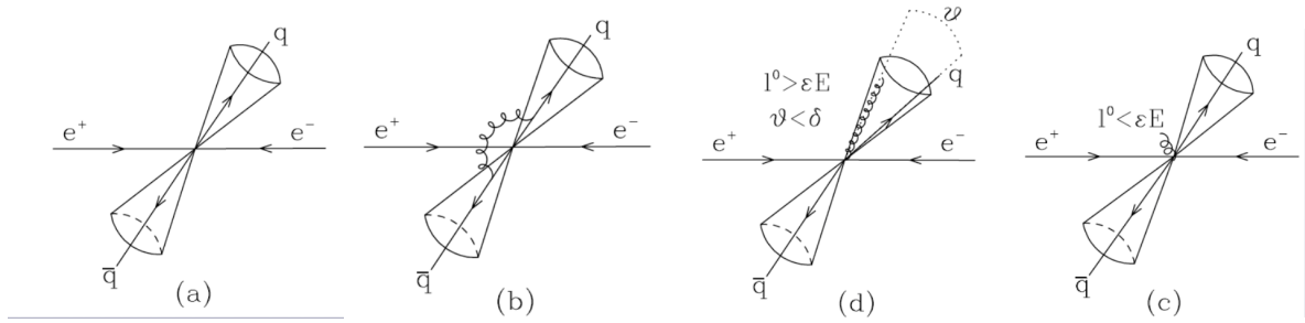
Figure 11: Diagrams for the various contributions to the QCD \alpha_s corrections to the calculation for the cross-section for the production of Sferman-Weinberg jets. From left to right we have the Born diagram, the virtual correction, and real emission falling both inside and outside the jet cone.
