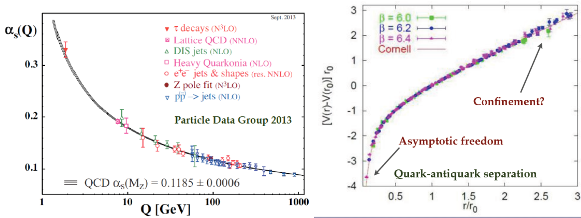
Figure 8: Left plot: summary of recent determinations of the QCD running coupling \alpha_s(Q) for different scales, together with the four-loops QCD prediction. Asymptotic freedom can be seen by the fact that \alpha_s(Q) decreases when Q is increased. Right plot: calculation of the potential between a quark-antiquark pair as a function of their separation, in lattice QCD.
