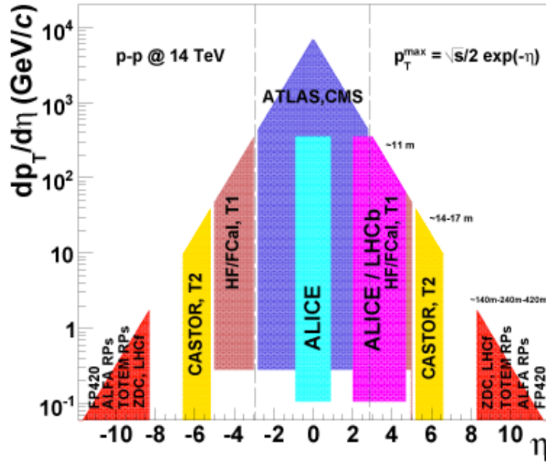
Figure 18: Approximate coverage in transverse momentum p_T and pseudo-rapidity \eta of current and future LHC detectors. For a given \sqrt{s} and pseudo-rapidity \eta , the kinematically maximum available p_T is p_T^{\max} \simeq \sqrt{s}e^{-\eta}/2 , as will be shown below.
