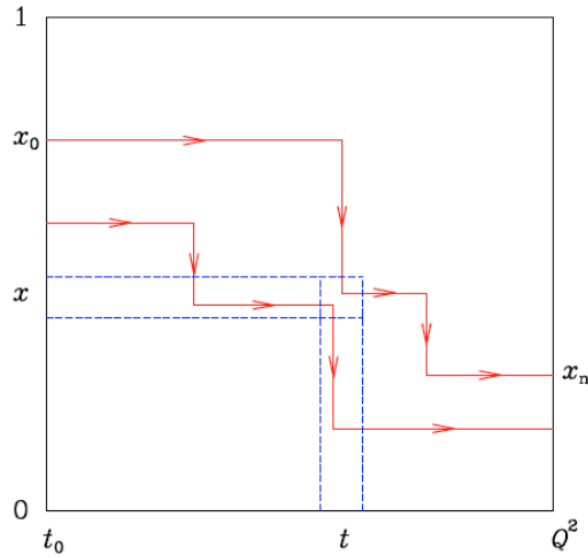
Figure 28: Path in the virtuality/momentum fraction plane for a initial state parton in a space-like shower from a low virtuality t_0 \simeq \Lambda_{\text{QCD}}^2 to the hard scattering virtuality t \simeq Q^2 . to high virtuality. See text for more details.
