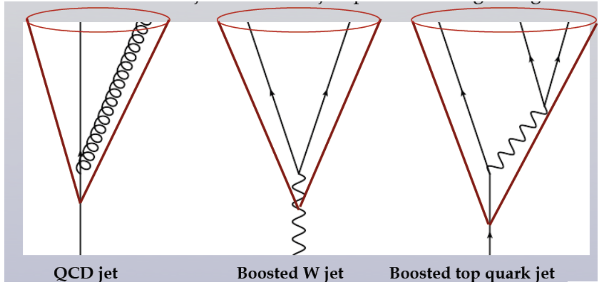
Figure 32: If a heavy resonance is produced with a large enough boost, p_T \gg m , then when decaying hadronically the final state becomes indistinguishable from that of QCD jets - unless one looks at the jet substructure.
