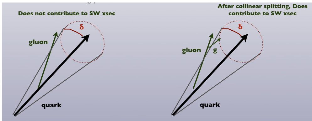
Figure 13: Origin of the IRC unsafety of the Sterman-Weinberg jets starting at \mathcal{O}(\alpha_s) .
