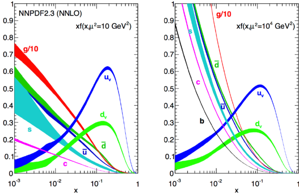
Figure 16: The NNPDF2.3NNLO set of parton distribution functions, at low scales \mu^2 = 10 \text{ GeV}^2 (left plot) and at a typical LHC scale \mu^2 = 10^4 \text{ GeV}^2 (right plot). The PDF evolution is completely determined by the perturbative DGLAP evolution equations. Note that the gluon PDF has been divided by 10 to be able to plot it using the same scale.
