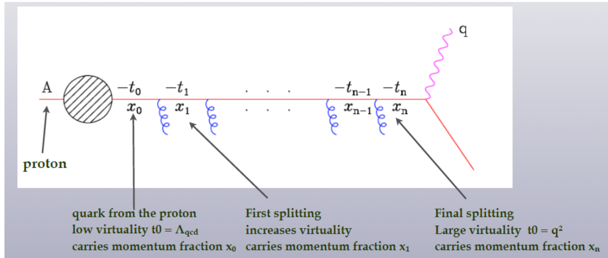
Figure 27: Schematic representation of a time-like parton shower branching, starting from a parton with low virtuality t_0 , which emits soft and collinear radiation under reaching the hard scattering virtuality.
