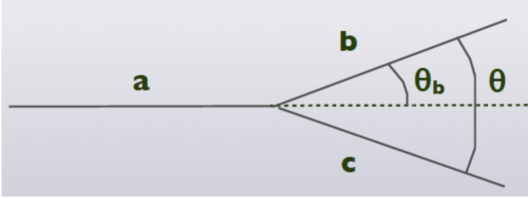
Figure 26: The collinear branching of a mother parton a into two daughter partons b and c .
