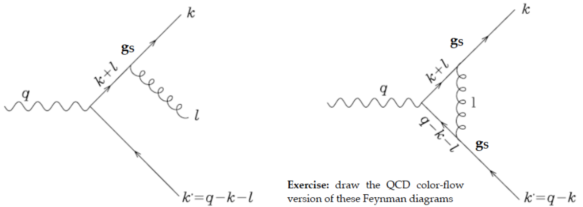
Figure 9: QCD corrections to quark-antiquark production in electron-positron annihilation. As an exercise, try to write the color-flow version of these diagrams.
