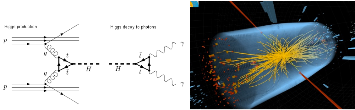
Figure 25: Left plot: Feynman diagram for the Higgs boson production in the gg channel, followed by a decay into di-photons. Right plot: a candidate CMS event for the same process.
