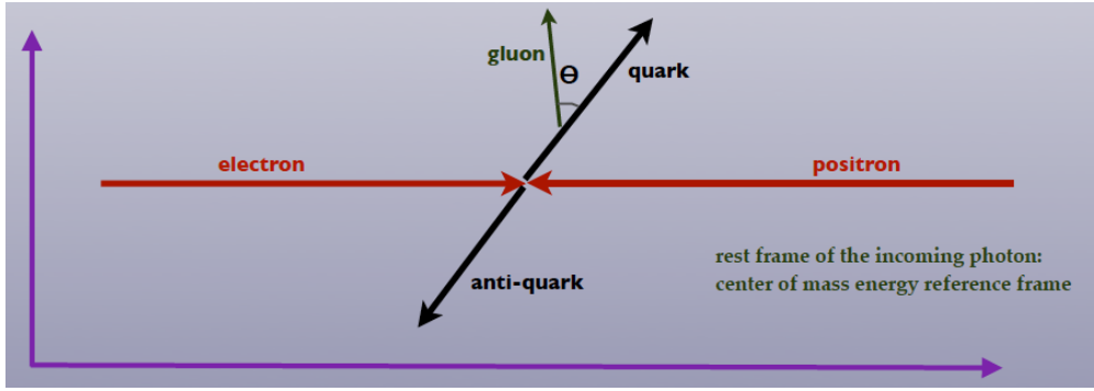
Figure 10: Kinematics of real gluon emission in quark-antiquark production via electron-positron annihilation.
