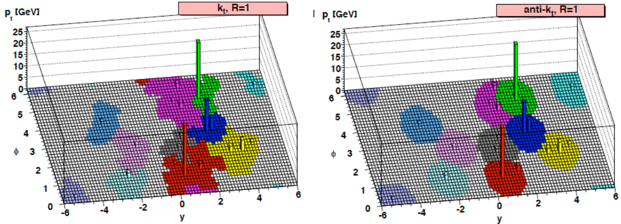
Figure 31: The catchment area of two jet algorithms, with R = 1 : the k_T algorithm and the anti- k_T algorithm. It is clear that the second produces much more regular jets than the first of the algorithms.
