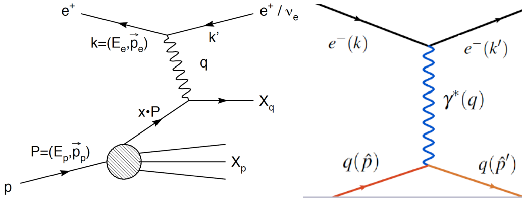
Figure 14: Left plot: the deep-inelastic scattering process. Right plot: the Born contribution to the lepton-quark scattering.
