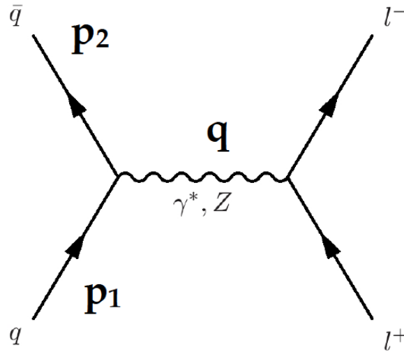
Figure 19: Feynman diagram for the hadroproduction of a neutral gauge boson, followed by the decay into two leptons, in the Born approximation. The four-momenta of the incoming quarks are labeled as p_1 and p_2 .
