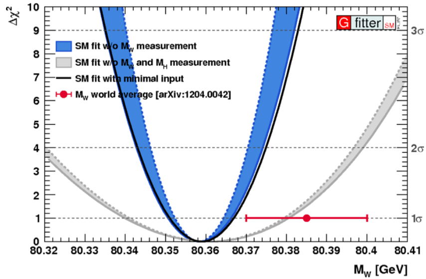
Figure 21: The impact of the direct W mass measurement in the global electroweak fit.
