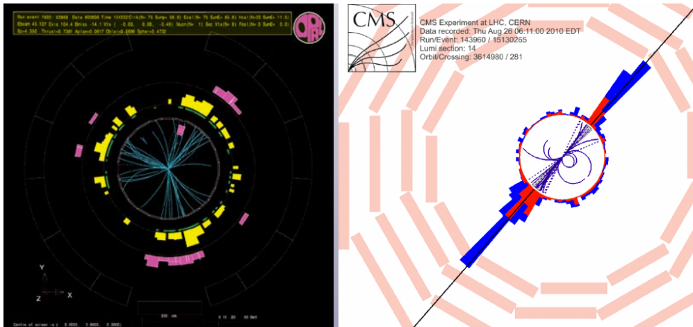
Figure 12: Left plot: discovery of the gluon in three-jet events from e^+e^- collisions at PETRA, in the late 70s. Right plot: high energy dijet event as measured by the CMS experiment at the LHC, for a center of mass energy of \sqrt{s} = 7 TeV.
