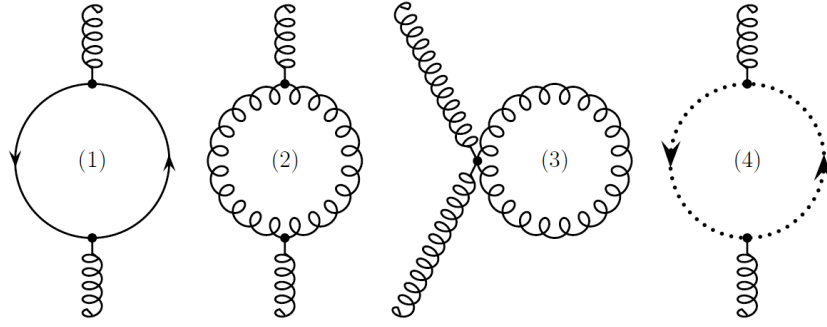
Figure 7: Feynman diagrams which contribute to the self-interactions of the gluon in QCD, and determine the leading order coefficient of the RGE equations for the running of \alpha_{\text{ren}}(\mu) in Eq. (53).
