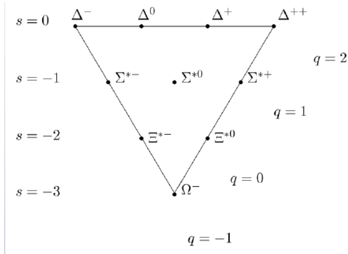
Figure 1: Upper plot: properties of quarks. Lower plot: the baryon decuplet with its various quantum numbers.
