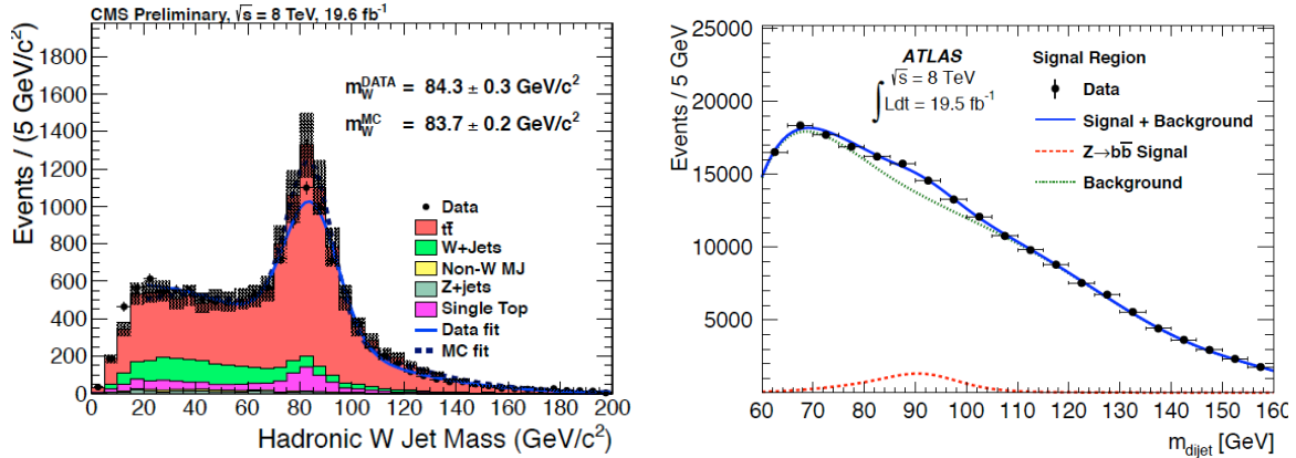
Figure 34: Left plot: in top quark pair decays, in a large fraction of events the W bosons decay hadronically. If the p_T is large enough, the hadronic decays of the W will be collimated into a single jet, which can then be reconstructed with substructure techniques, resulting in a nice peak around the W mass for the the jet invariant mass. Right plot: ATLAS has managed to reconstruct the Z \rightarrow b\bar{b} decays in events where the Z boson carries large transverse momentum, and where jet substructure techniques allow to identify this decay channel over the overwhelming QCD background.
