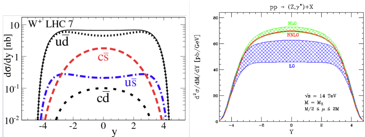
Figure 20: Left plot: the contribution of different partonic initial states to the rapidity distribution of W^+ bosons at the LHC 7 TeV. Right plot: the calculation of the rapidity distribution of Z bosons at the LHC 14 TeV, computed at LO, NLO and NNLO accuracy. The bands represent the theoretical uncertainty in the calculation arising from higher orders.
