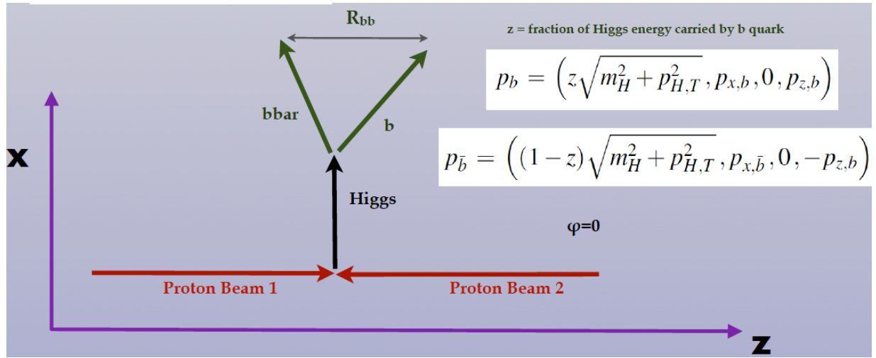
Figure 33: Scheme for the central production of a Higgs boson in a hadronic collision, followed by the decay into a b\bar{b} pairs.
