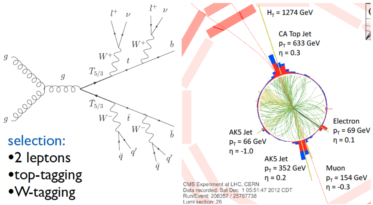
Figure 35: Feynman diagram which correspond to the pair production of fermionic top partners (that would arise for example in models where the Higgs boson is a composite particle) and that might contain a number of fast jets in the final state, in particular from the hadronic decays of W bosons.
