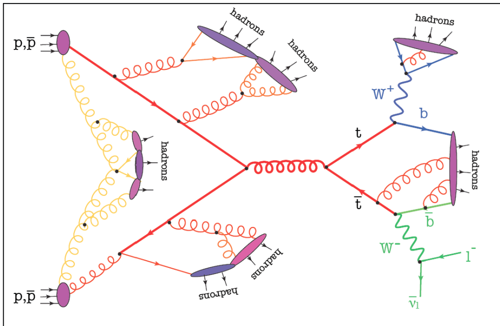
Figure 29: Schematic representation of the various ingredients that enter an hadronic collision, from the initial state (parton distributions) to the hard scattering cross-section to the final state (parton shower, hadronization), and then supplemented by non-perturbative soft physics for the underlying event and multiple parton interactions (Drawing by K. Hamilton).
