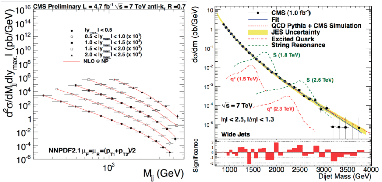
Figure 23: Left plot: the CMS measurement of the dijet cross-section at 7 TeV, compared with NLO QCD predictions with the NNPDF2.1 set. Right plot: the same observable, now used to search for New Physics that would appear as bumps in the otherwise smooth distribution due to new exotic particles being produced.
