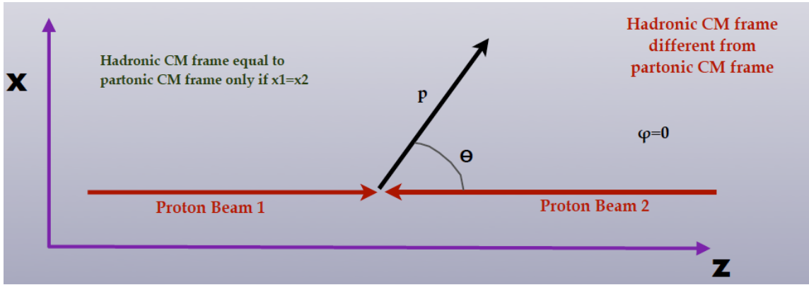
Figure 17: Kinematics of an hadron-hadron collision for an azimuthal angle of \phi = 0 . In general, the hadronic center of mass frame will be different to the partonic center of mass frame.
