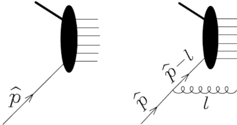
Figure 15: Left plot: the DIS matrix element calculation at Born level. Right plot: same as before but now accounting for the radiation of an additional gluon from the initial state quark.
