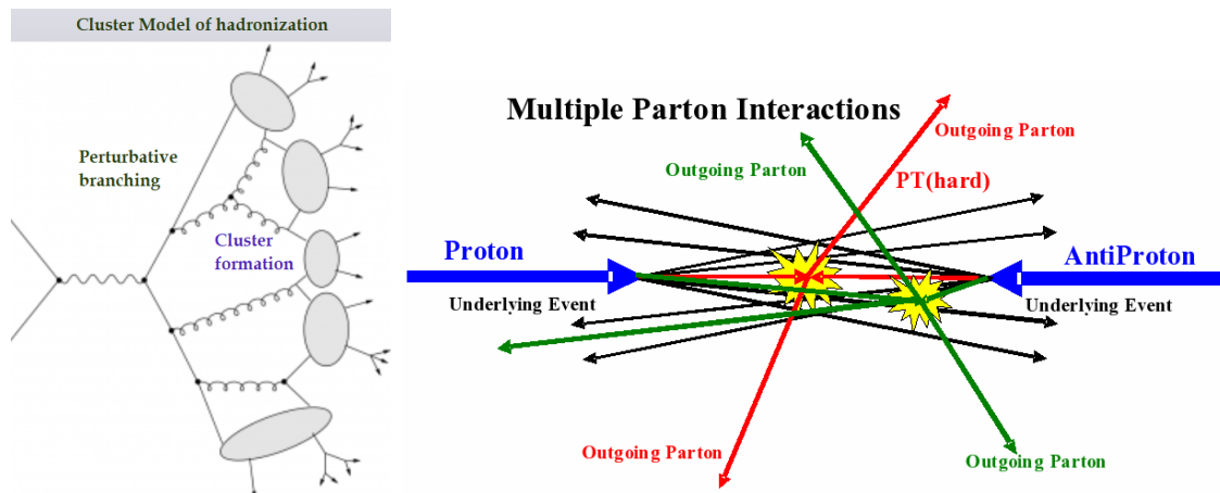
Figure 30: Left plot: schematic representation of the cluster model of hadronization, where a cluster formation step follows the perturbative parton branching process. Right plot: schematic representation of multiple parton interactions at an hadron collider.
