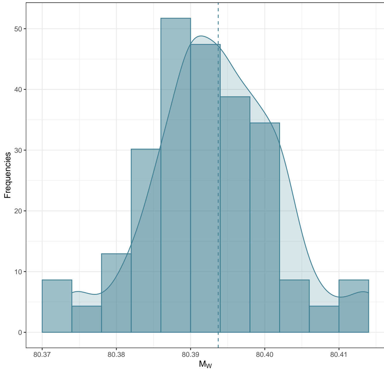
Mw Dist. using CT18 in Pseudodata & NNPDF40 in Templates
