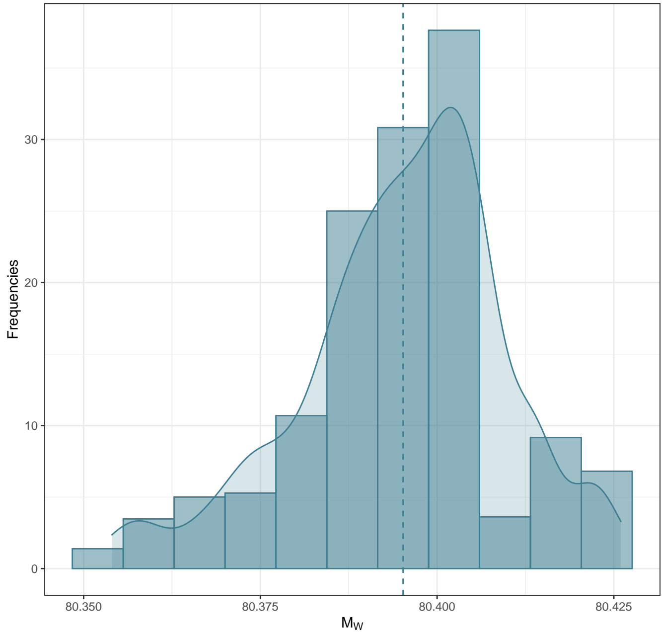
Mw Dist. using NNPDF40_1000 in Pseudodata & NNPDF31 in Templates
