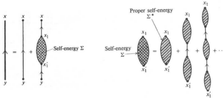
Figure 3: Graphical definition of the self-energy. Google Images
